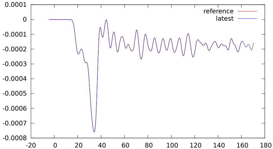
XS.S001.MXE.sem.ascii
