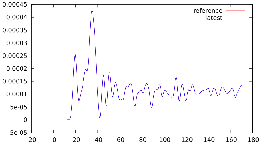
XS.S001.MXZ.sem.ascii
