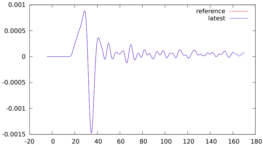
XS.S001.MXN.sem.ascii
